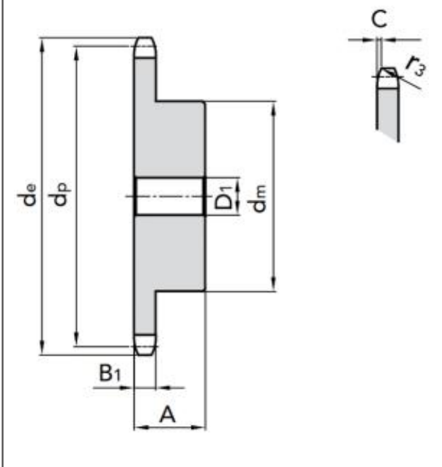
2D Technical Drawing
